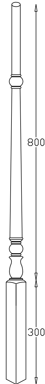
Spindle 1100mm
