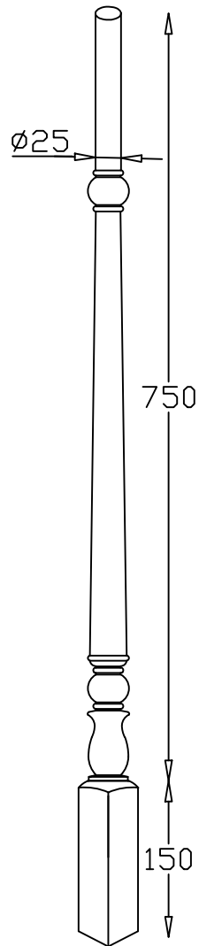
Spindle 900mm
